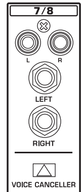
Fig. 3.2: Stereo channel connectors
