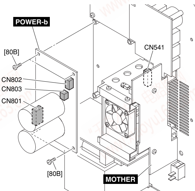
[80B]: BIND HEAD SCREW 3.0x8 CR3 (AAX61910) 小ネジ + BIND
