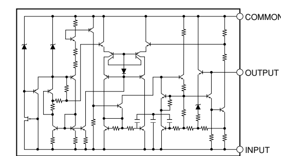
IC14: NJM79M12FA Voltage Regulator
