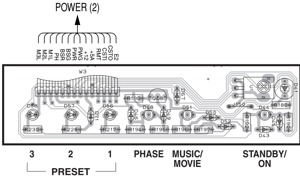
POWER (3) P. C. B. (Lead Type Device)
