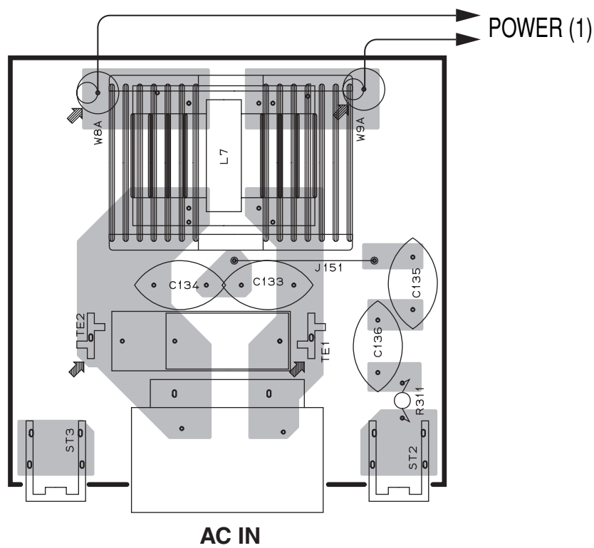
INLET P. C. B. (Lead Type Device)
