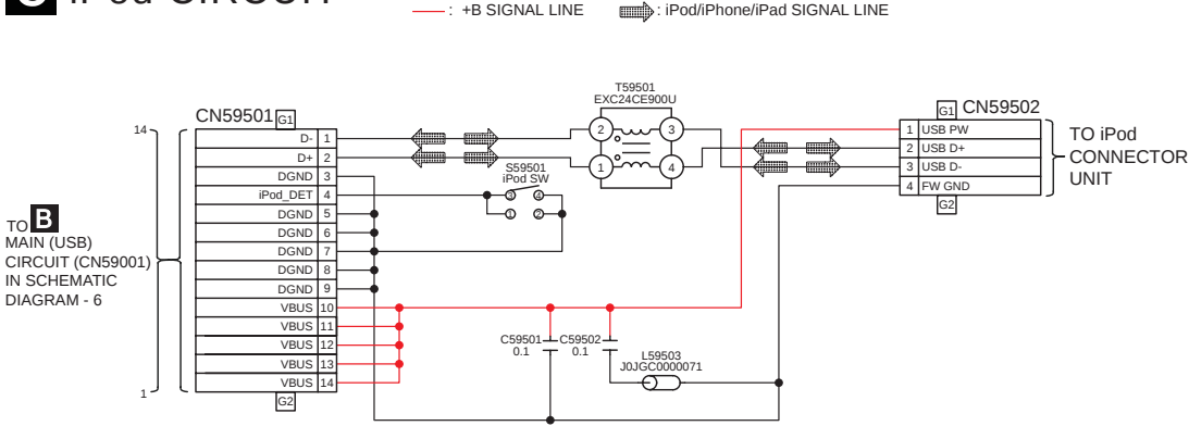
SCHEMATIC DIAGRAM - 8
