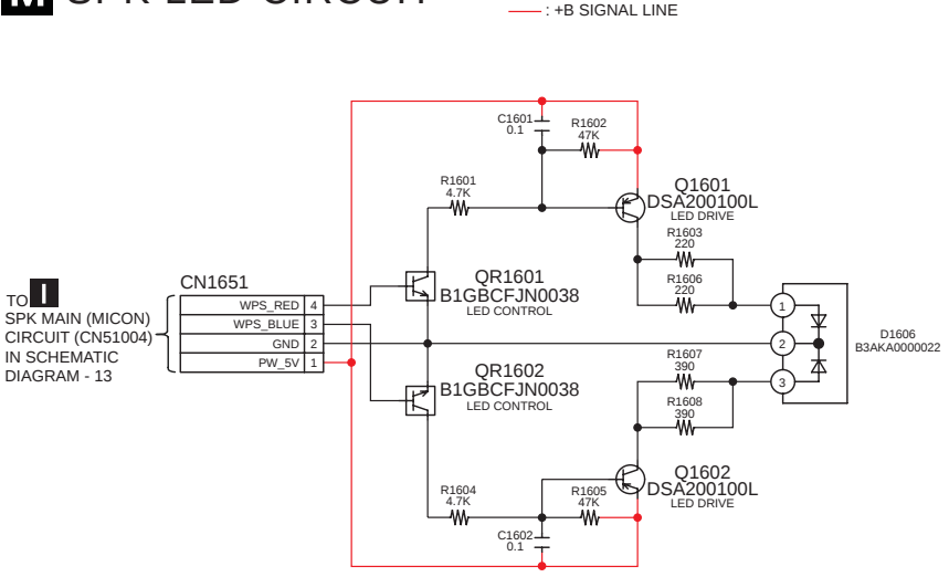
M SPK LED CIRCUIT
