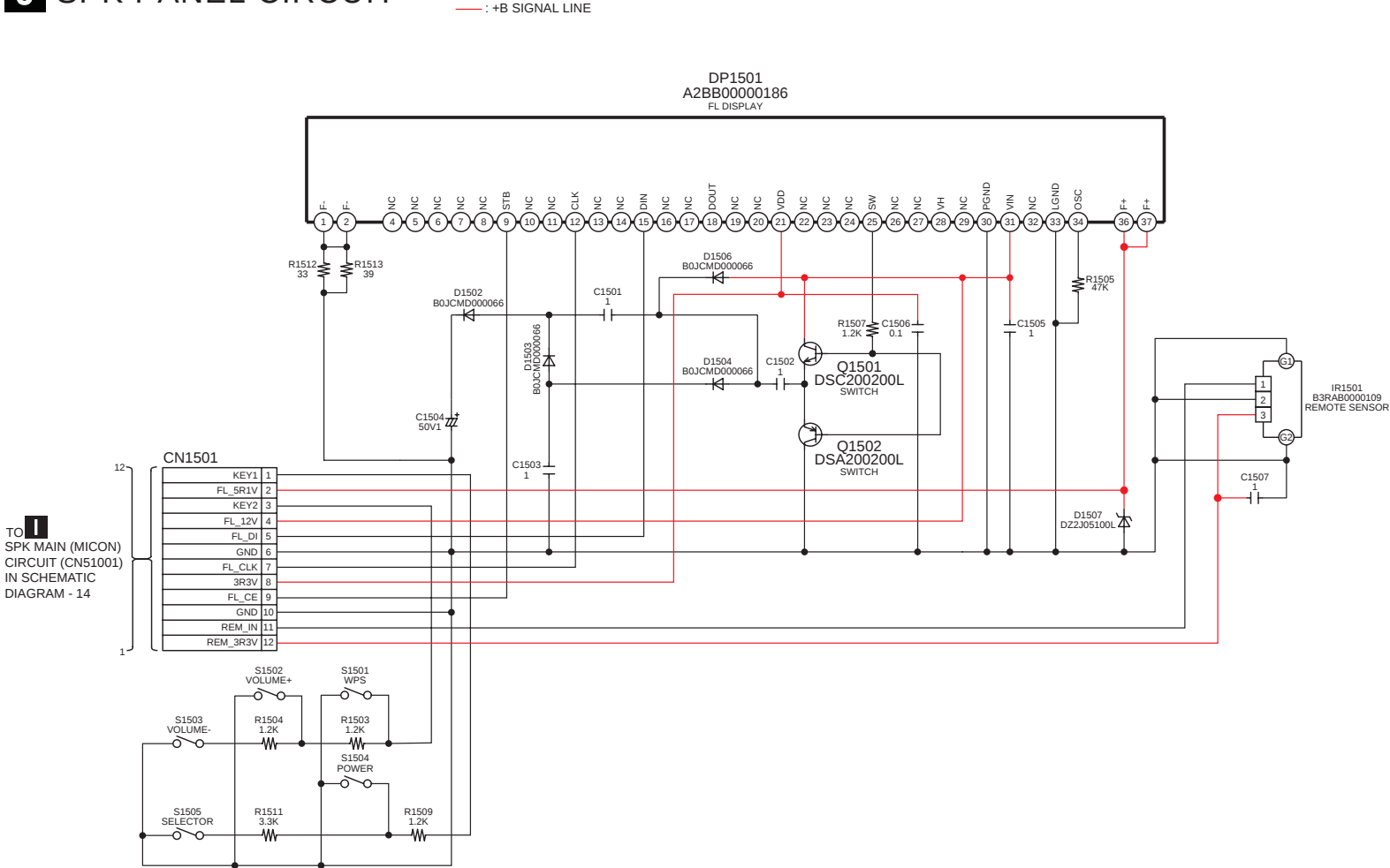
SCHEMATIC DIAGRAM - 18 J SPK PANEL CIRCUIT
